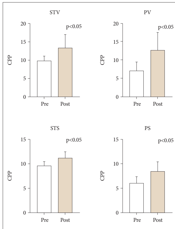
Supplementary Fig. 3. Pre-post injection laryngoplasty & arytenoid adduction treatment CPP value comparison. STV, speech tool vowel; PV, Praat vowel; STS, speech tool sentence; PS, Praat sentence; CPP, cepstral peak prominence.
